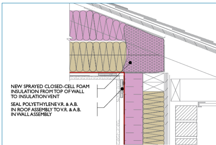
Figure 5: Roof at wall—sprayed closed-cell foam
