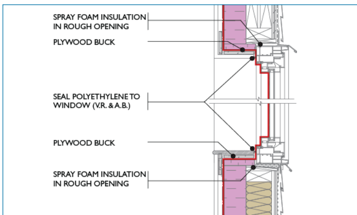
Figure 8: Polyethylene air barrier sealed to the inside of the window
