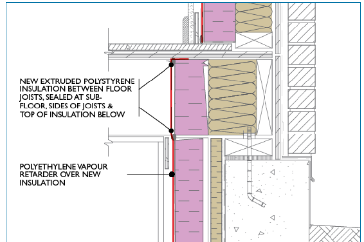
Figure 10: Rim joist—polystyrene insulation
