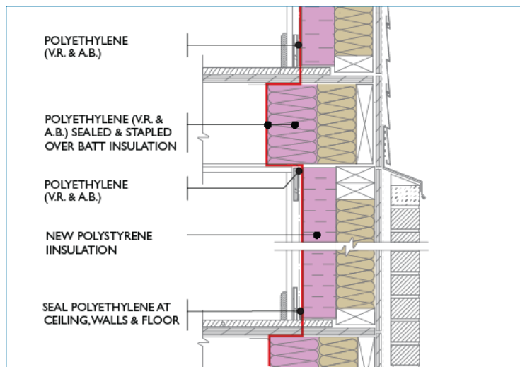
Figure 7: Above-grade walls—insulation and air sealing inboard of stud-frame wall
