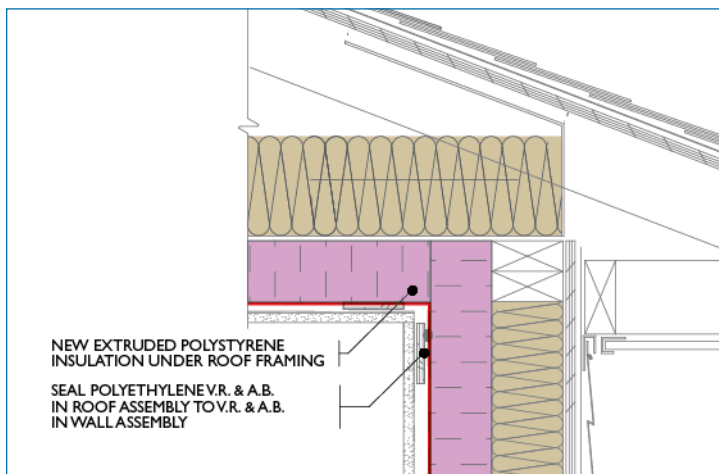
Figure 6: Polystyrene added under roof framing
