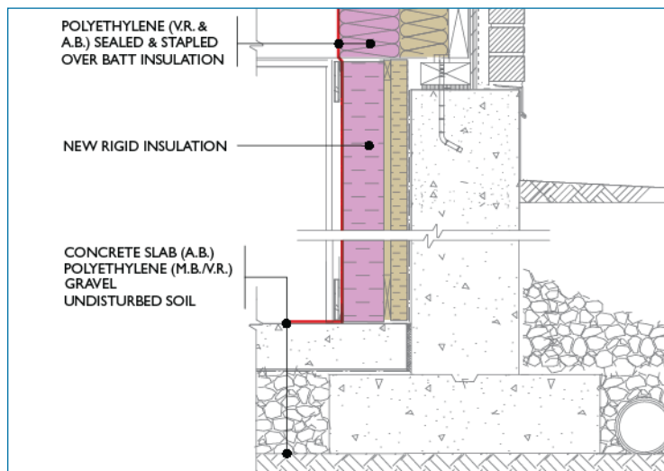
Figure 9: Below-grade walls—insulation and air sealing inboard of foundation wall
