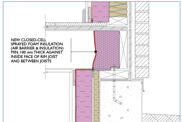
Figure 11: Rim joist—closed-cell sprayed foam
