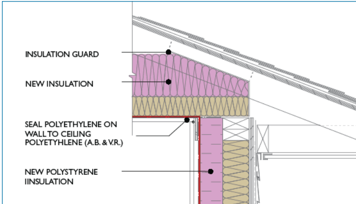
Figure 4: Roof and attic—closed-cell sprayed insulation at eaves
